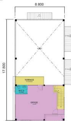
TYPE B: FIRST FLOOR PLAN
