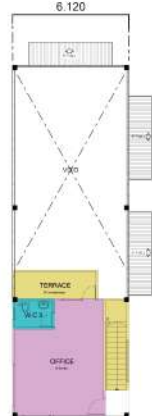
TYPE A: FIRST FLOOR PLAN
